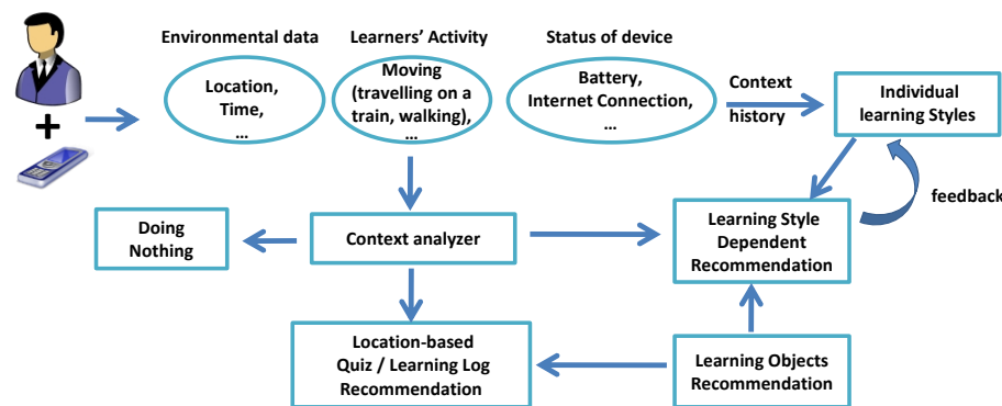
Figure 1: Workflow of the personalization and context-awareness model
