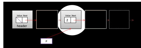
Fig. 2 Model of linked list with highlighting function
