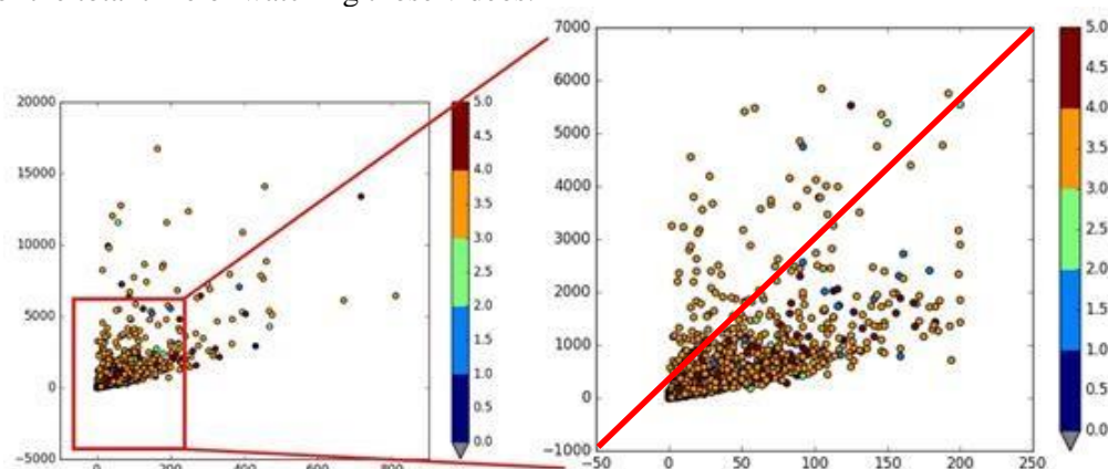
Figure 2. Result of Clustering Analysis
