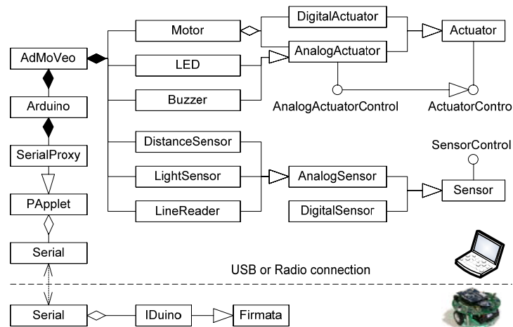
Fig. 2 Software Architecture
