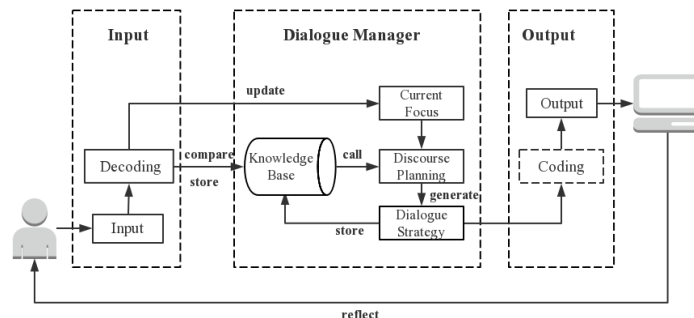
Figure 18. Architecture of Collaborative Problem Solving Supported Conversational Agent (CP2SCA)
