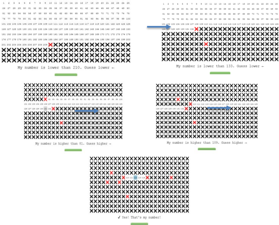
Figure 1. Example of incremental binary search
