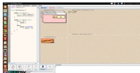
Figure 3: Codeasy- Java visualization tool
