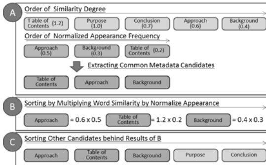
Figure 2. Recommendation Algorithm
