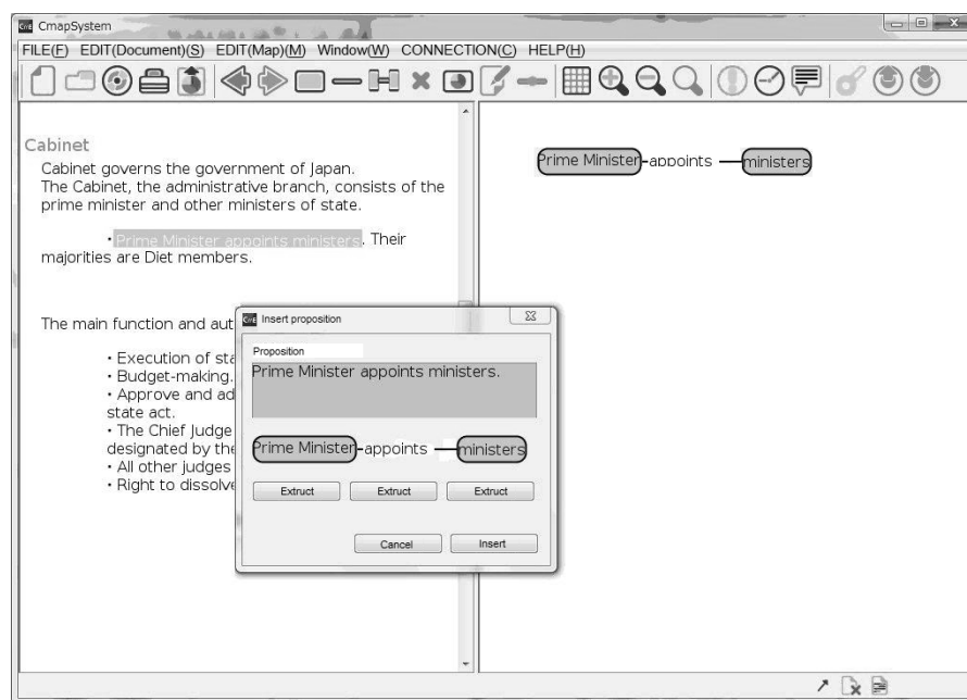
Figure 1: CmapEditor
